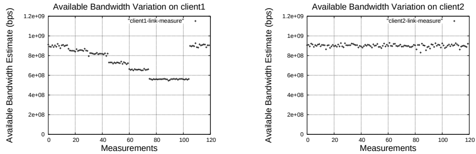
(a) Available bandwidth on client1 varies much like router1 and router3 , as the download rate changes
