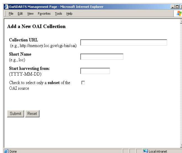
Figure 5: The user interface for “wrapping” an OAI collection and make it SDARTS compliant.
