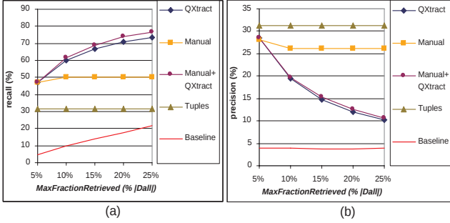
Figure 12. Recall (a) and precision (b) of QXtract, Tuples, Manual, Manual+QXtract, and Baseline over the test database using Proteus as the target information extraction system (DiseaseOutbreaks relation).
