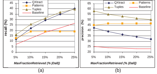
Figure 10. Recall (a) and precision (b) of QXtract , Patterns , Tuples , and Baseline over the test database using DIPRE as the information extraction system ( Headquarters relation).
